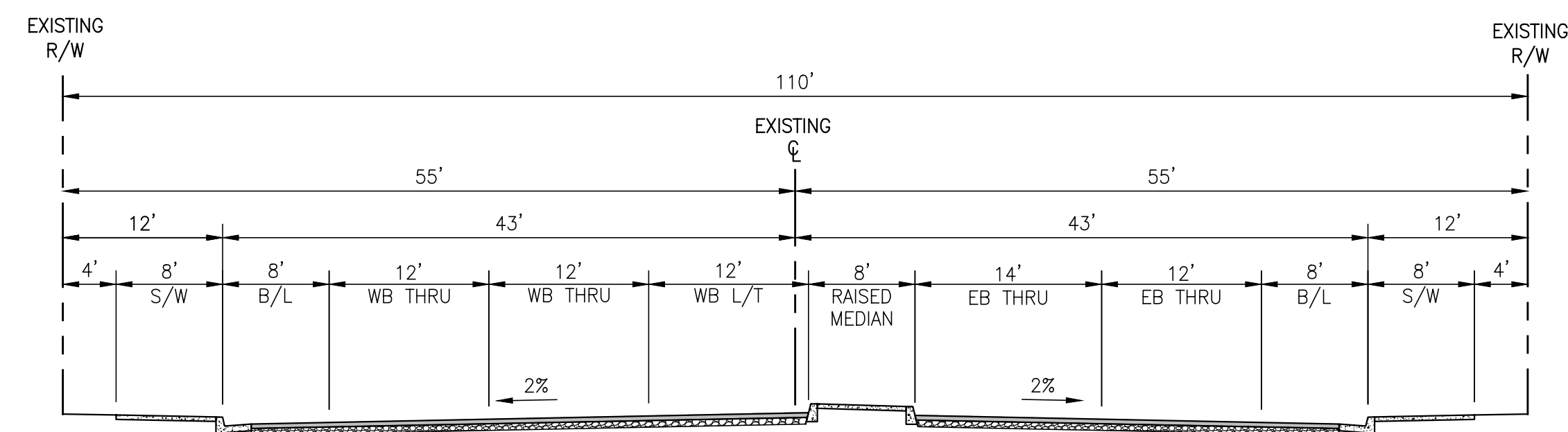
SECTION F-F PROPOSED SUN LAKES BOULEVARD (EASTERLY INTERSECTION APPROACH AT FUTURE STREET) ARTERIAL HIGHWAY SCALE: 1" = 10'
